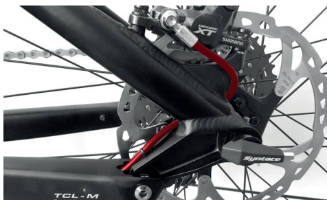
Picture shows rear brake on a Post Mount socket with hose routing for Shimano.
